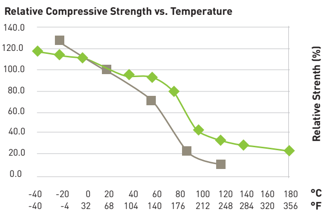
Figure 2: Relative compressive strength vs. temperature.
