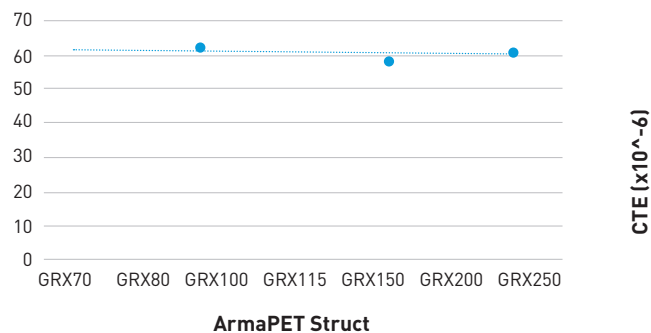
Figure 6: CTE vs. foam density
