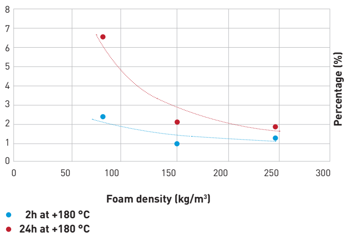
Figure 8: Shrinkage in Z direction (%) at +180 °C
