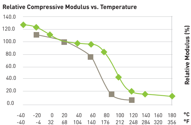
Figure 1: Relative compression modulus vs. temperature.
