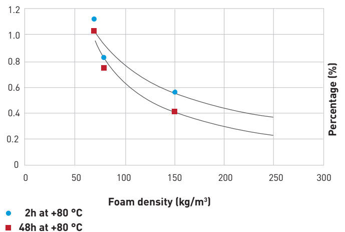
Figure 7: Shrinkage in Z direction (%) at +80 °C
