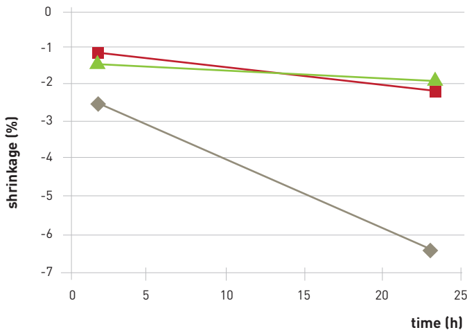
Dimensional Stability vs. Time at 180°C, 1 bar / 356°F, 14.5 psi
