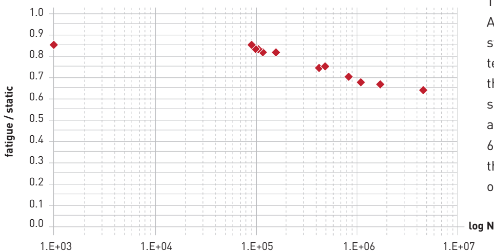
Caption: Normalized S-N diagram for ArmaPET Struct GRX115
