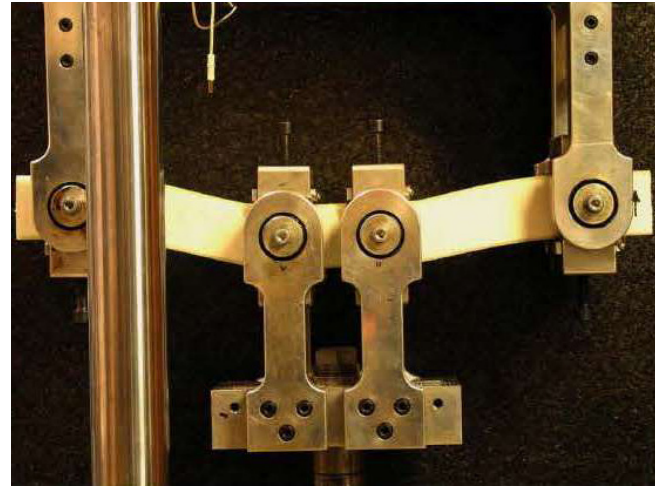
Caption: Four-point bending set-up
