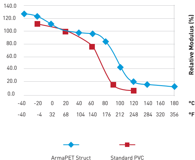
Relative Compressive Strength vs. Temperature
