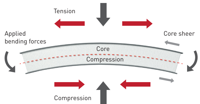
Caption: Stress in sandwich panels
