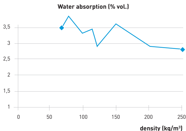
Caption: Water absorption in % vol. for a 28 days immersion in function of the density
