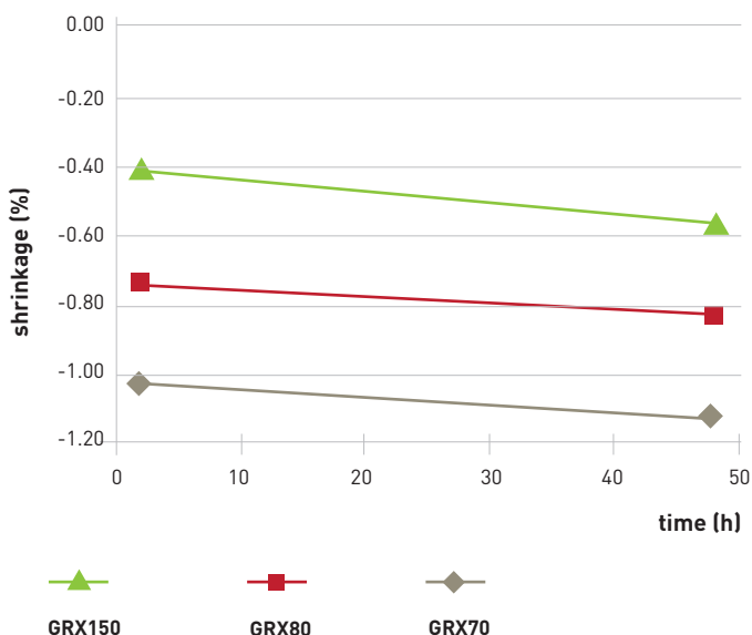
Dimensional Stability vs. Time at 80^{\circ}\text{C} , 1 bar / 14.5 psi, 176^{\circ}\text{F}
