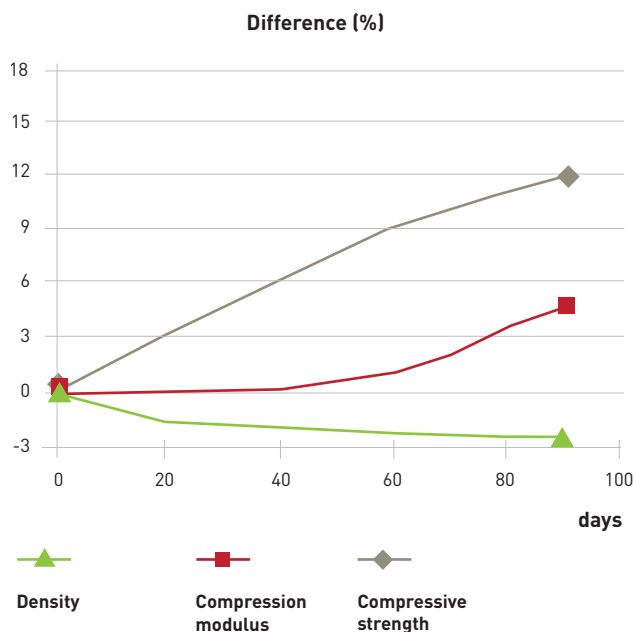
Caption: Difference (in %) of different properties in function of the exposition time to UV (in days) compared to day 0 for Eco50
