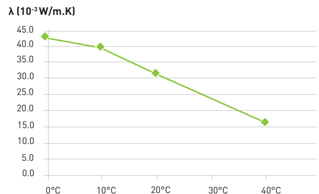
Thermal Conductivity vs. Temperature (ArmaPET Struct GRX70)
