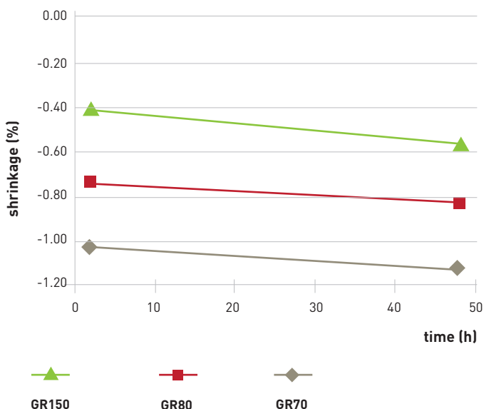
Dimensional Stability vs. Time at 80°C, 1 bar / 14.5 psi, 176°F
