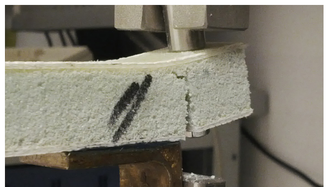
Figure 4: Peel off test on a sample
